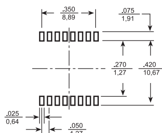
SUGGESTED LAND PATTERN
